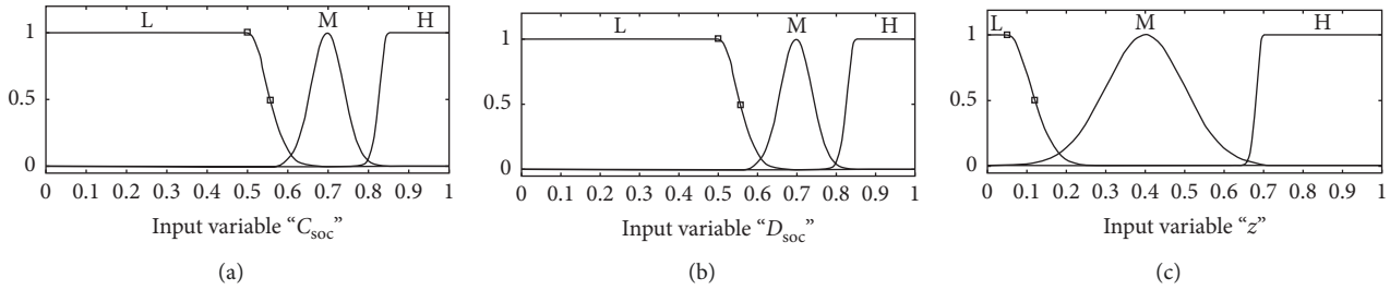
FIGURE 10: Input membership function of the middle braking strength fuzzy controller.
