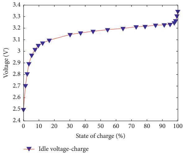
FIGURE 15: Battery characteristics.
