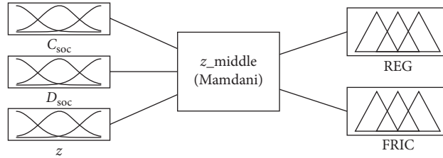
FIGURE 9: Middle braking strength fuzzy controller structure.
