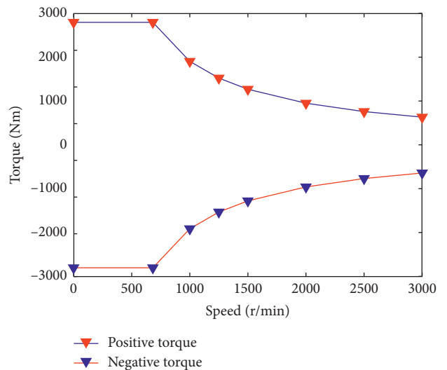
FIGURE 14: Motor characteristics.
